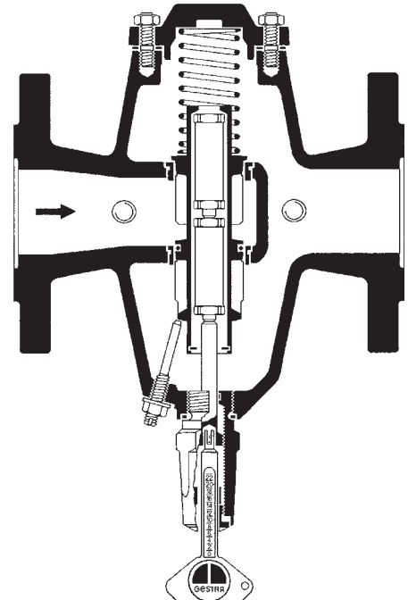
CW 41 DN 40/50
